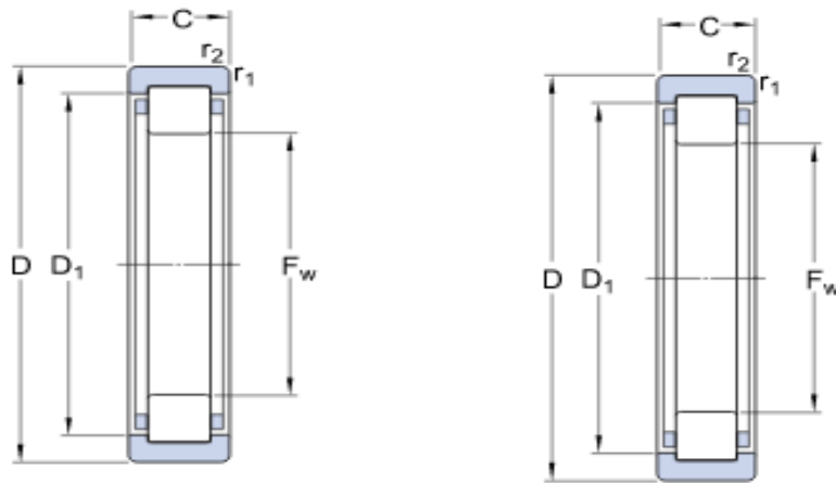
No inner Ring Cylindrical Roller Bearing
